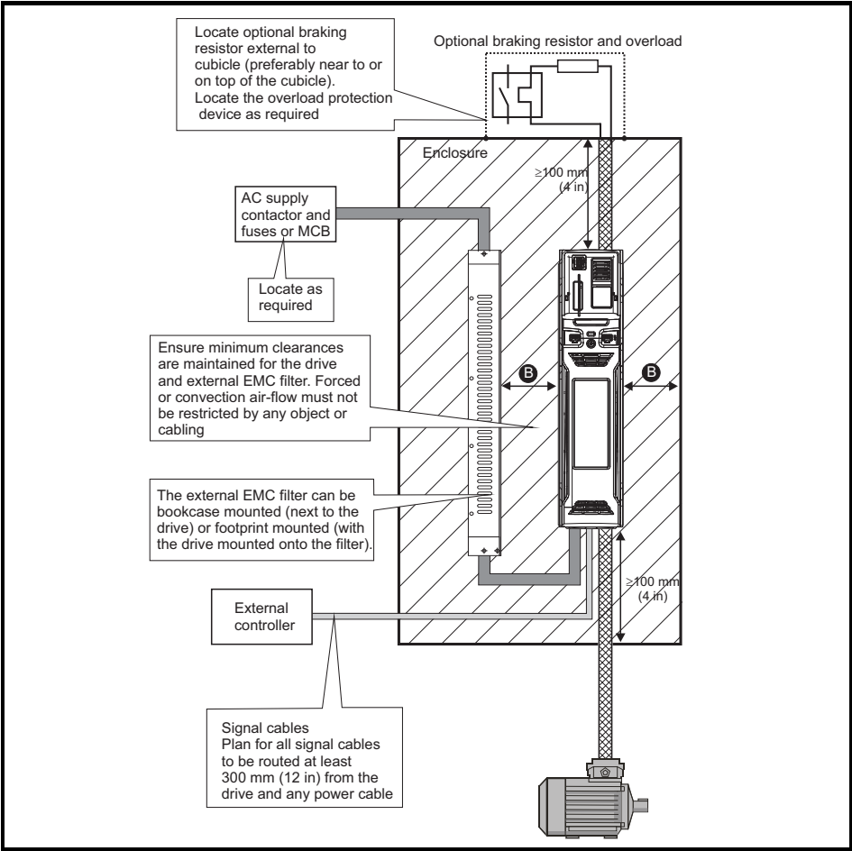
Figure 3-11 Enclosure layout
