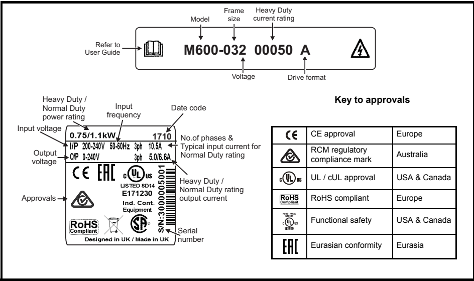
Figure 2-2 Typical drive rating labels (Unidrive M600 labels illustrated)
